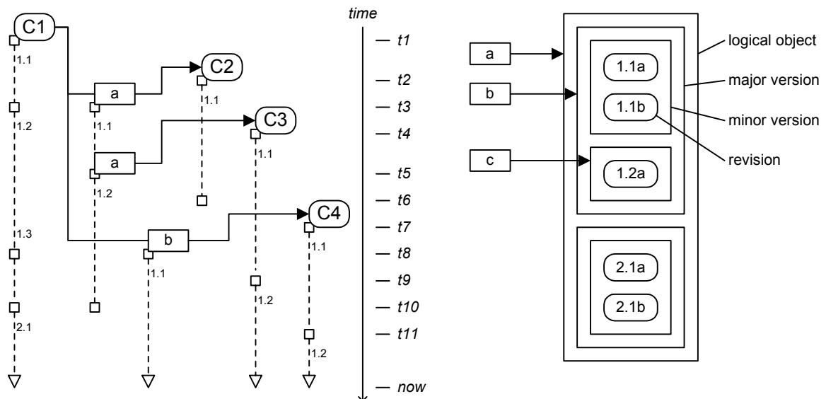
Figure 2 Left: example of a timeline of concept versions. At moment t_5 , the relationship a from concept C_1 to concept C_2 is changed into a relationship to concept C_3 . Although this does not lead to a new version of concept C_1 , this change can be traced through the concept's timeline.
