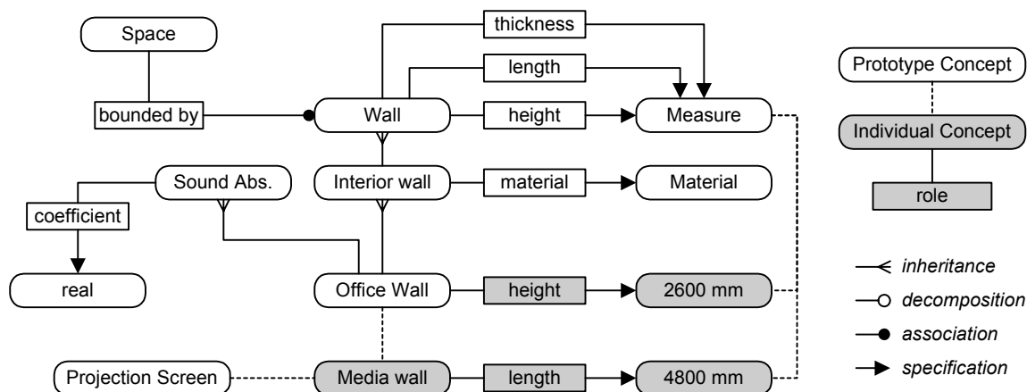
Figure 1 Example of a network of concepts. The prototype concept ‘Office Wall’ inherits from the ‘Interior Wall’ and the ‘Sound Absorbing Element’ concepts. It overrides the inherited ‘height’ relationship by fixing it to 2600 mm. The ‘Media Wall’ is an individual concept based on the prototype ‘Office Wall’ of which it uses the height; the length is added to this individual. The ‘Media Wall’ also implements the prototype ‘Projection Screen’ (no further details shown here).
