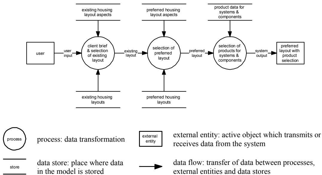
Figure 2. Decision Support System Process Model
